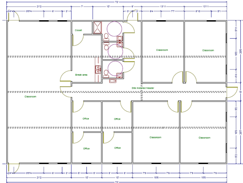
Proposed floor plan for the new modular building at Palma Nova
